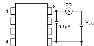
Fig. 13.1.6 I CCL Test Circuit
