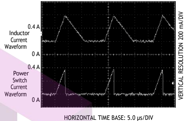
Figure 24. Discontinuous Mode Switching Current Waveforms
