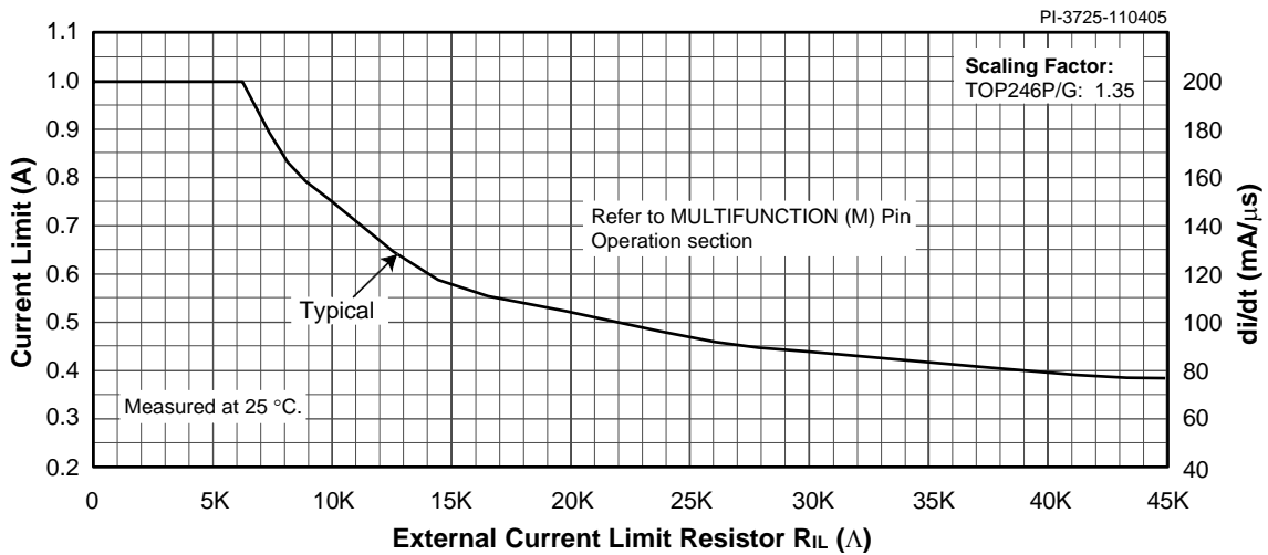
Figure 56b. Current Limit vs. External Current Limit Resistance (TOP246P/G only).
