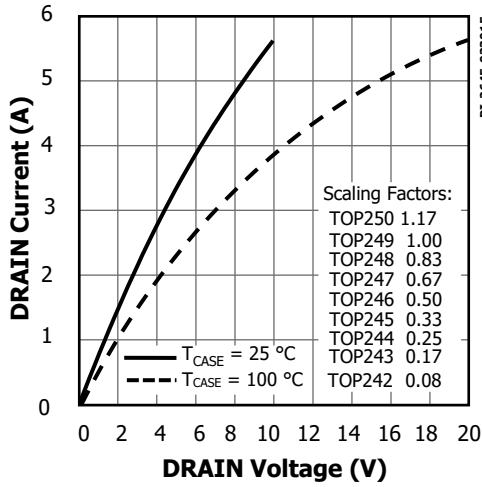
Figure 67. Output Characteristics.
