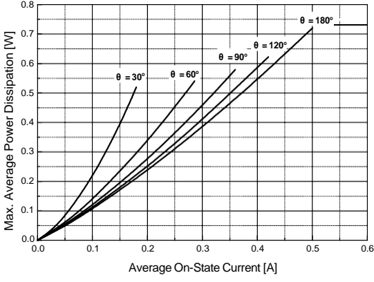
Fig 8. Power Dissipation
