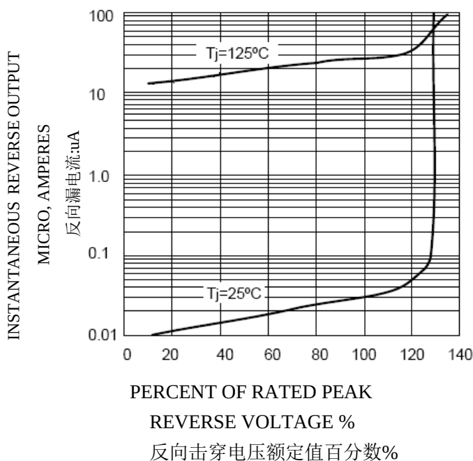
FIG.3 TYPECAL REVERSE CHARACTERISTICS PER BRIDGE ELEMENT
