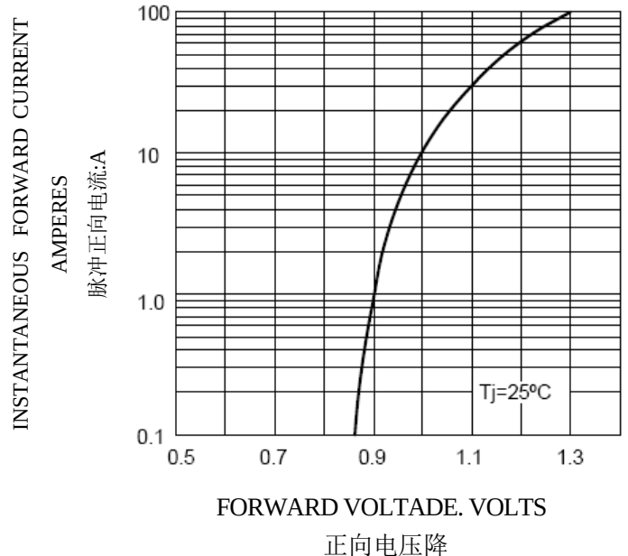
FIG.4 TYPECAL FORWARD CHARACTERISTICS PER BRIDGE ELEMENT
