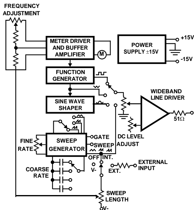
FIGURE 10D. INTERCONNECTIONS
