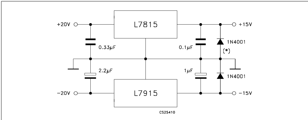
Figure 16. Split power supply (± 15 V - 1 A)
