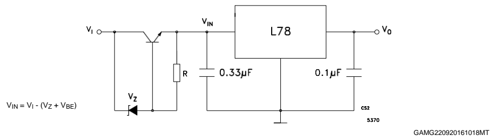
Figure 20. High input voltage circuit (configuration 1)
