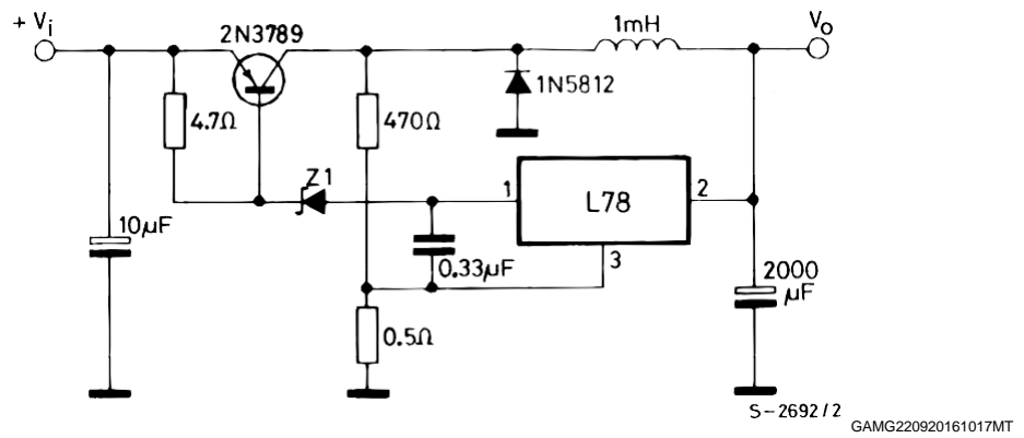
Figure 20. High input voltage circuit (configuration 1)
