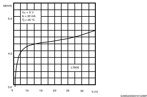
Figure 37. Quiescent current vs. input voltage
