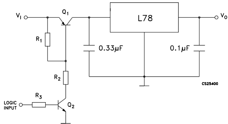
Figure 24. Remote shutdown
