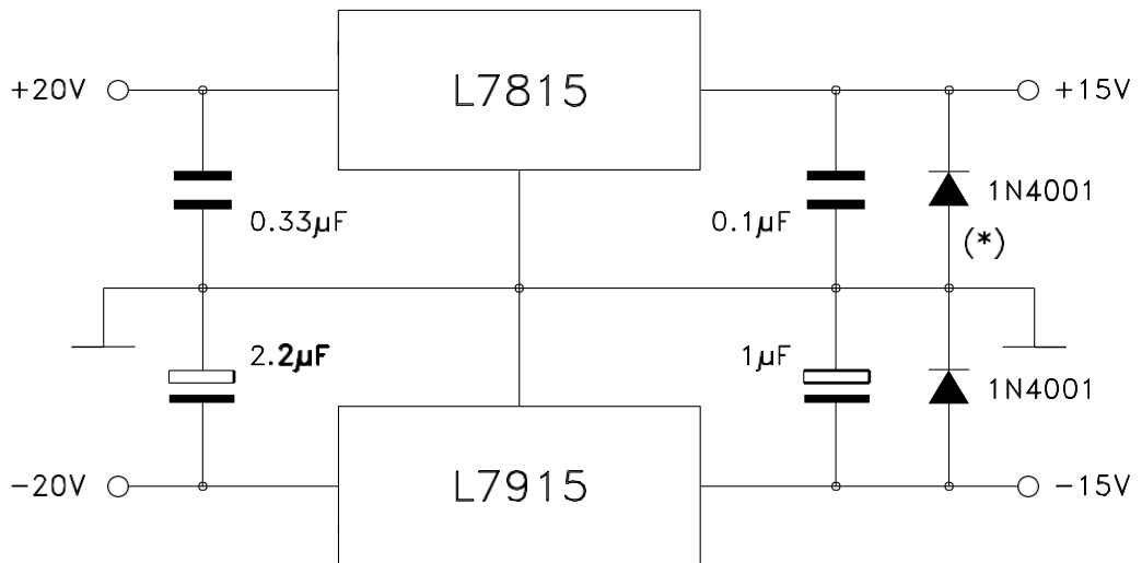
Figure 17. Split power supply ( \pm 15\text{ V} - 1\text{ A} )
