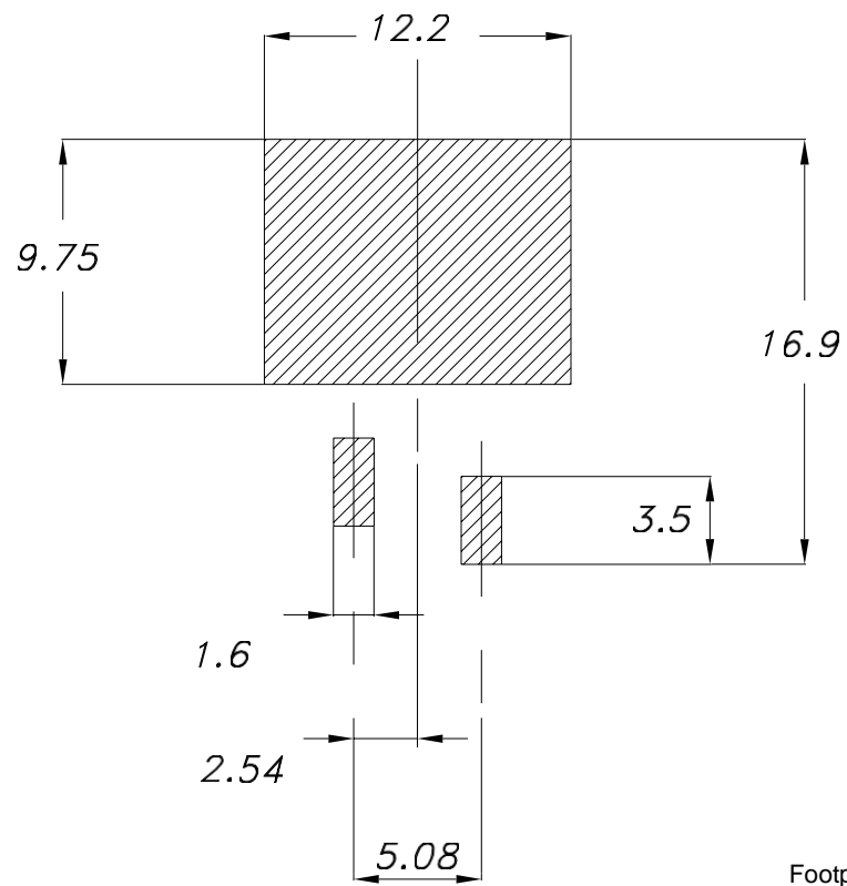
Figure 47. D 2 PAK recommended footprint (dimensions are in mm)
