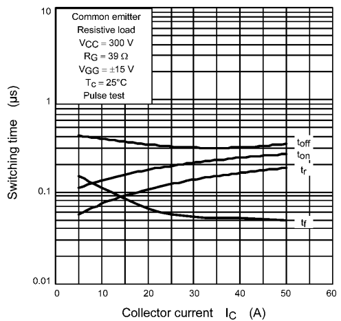
Fig. 8.6 Switching Time - I_C
