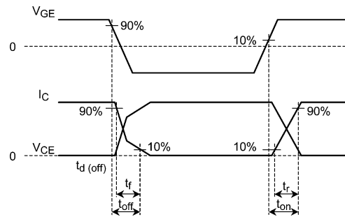
Fig. 6.2.2 Timing Chart of Switching Time
