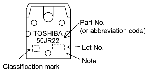
Fig. 7.1 Marking
