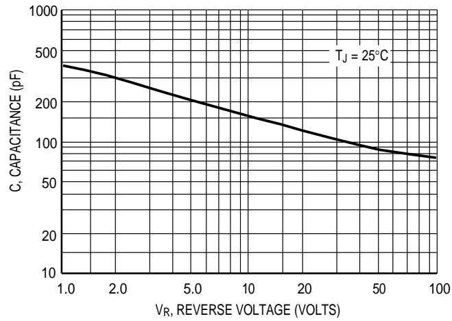
Figure 20. Typical Capacitance
