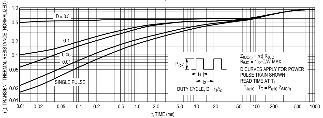
Figure 17. Thermal Response
