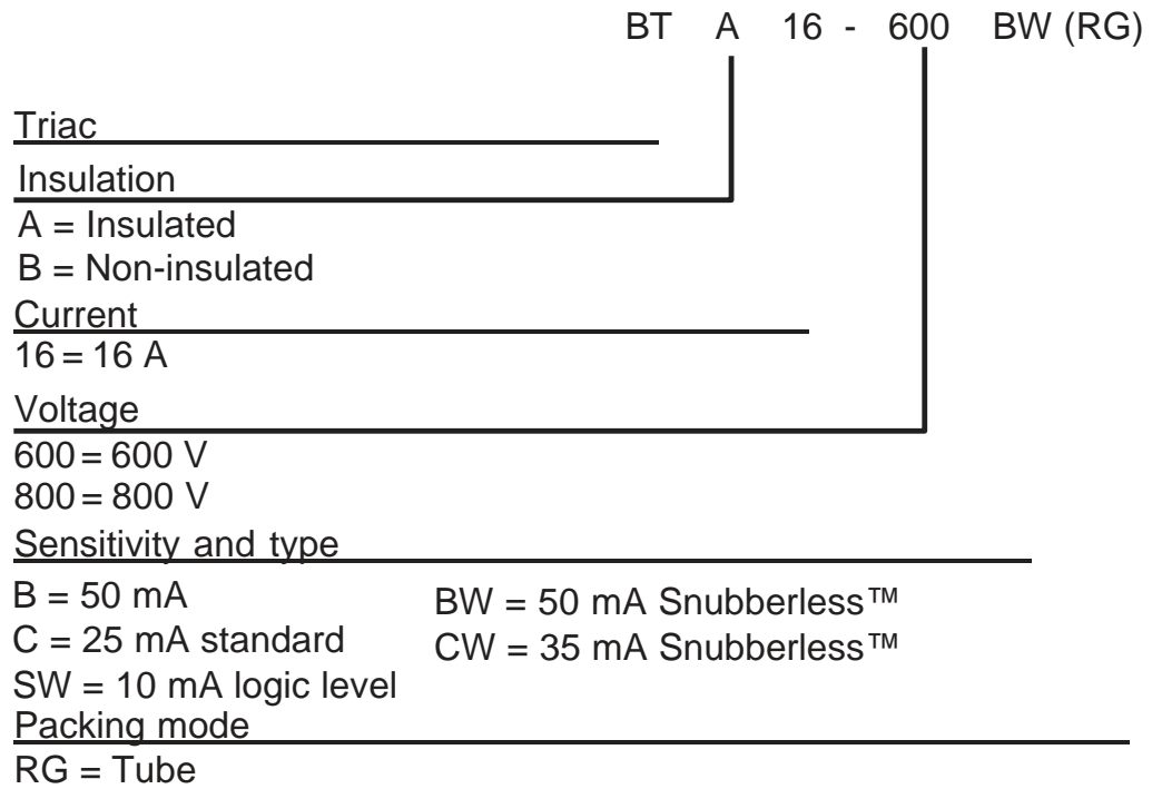
Figure 16. Ordering information scheme (BTA16 and BTB16 series)
