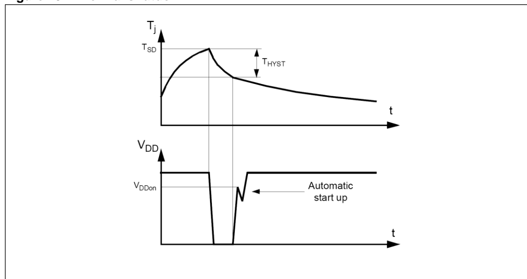
Figure 13. Thermal shutdown
