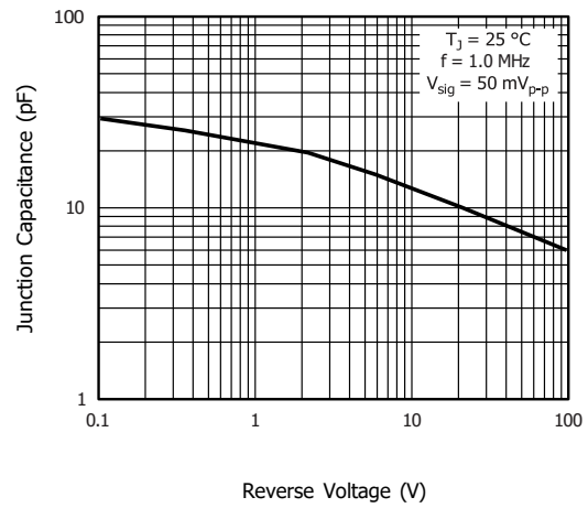
Fig. 7 - Typical Junction Capacitance
