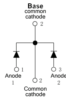
TO-3PB
