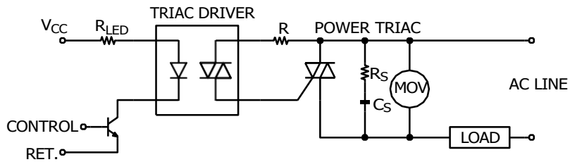
Figure 7. Basic Driver Circuit
