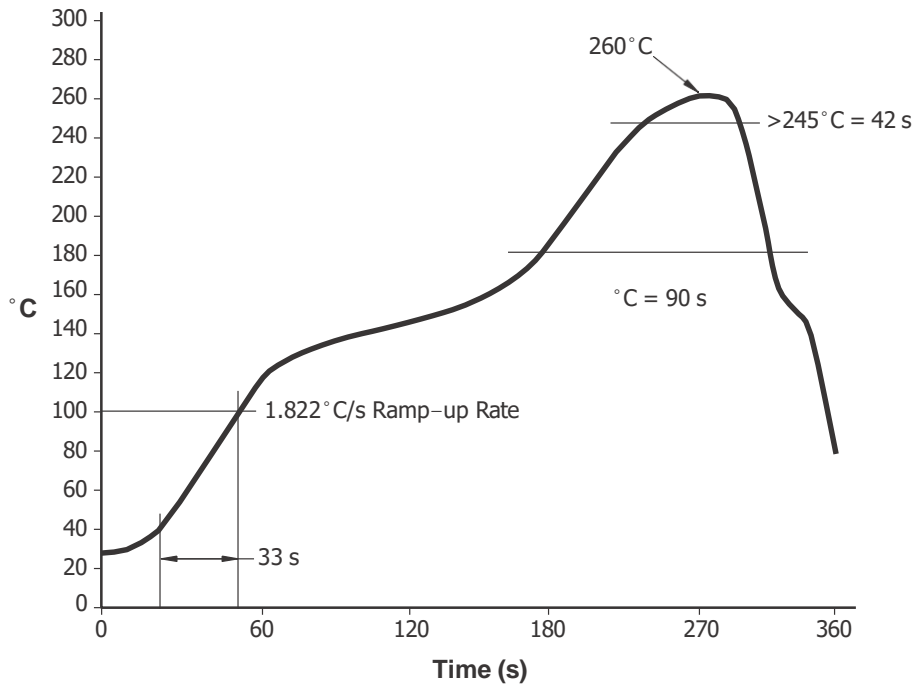
Figure 9. Reflow Profile
