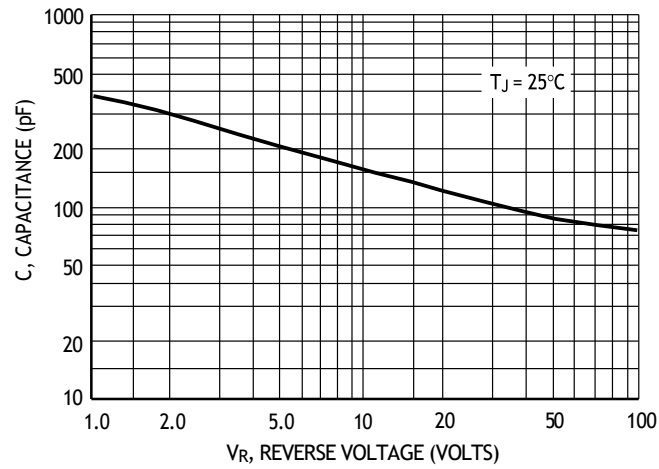
Figure 17. Typical Capacitance
