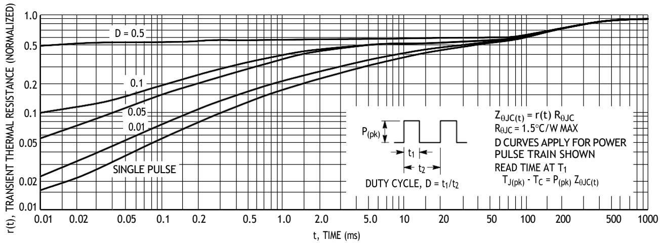
Figure 16. Thermal Response
