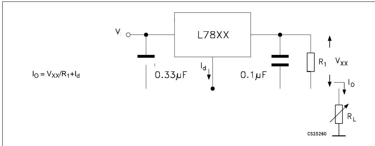
Figure 9. Current regulator
