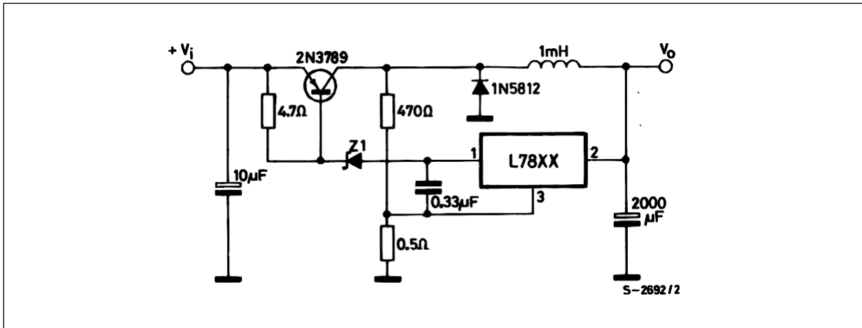
Figure 18. Switching regulator
