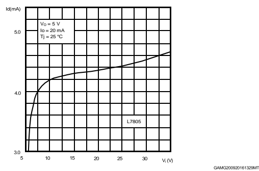
Figure 36. Quiescent current vs. input voltage
