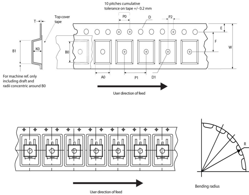
Figure 47. Tape outline
