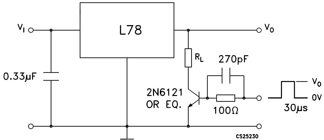
Figure 6. Load regulation
