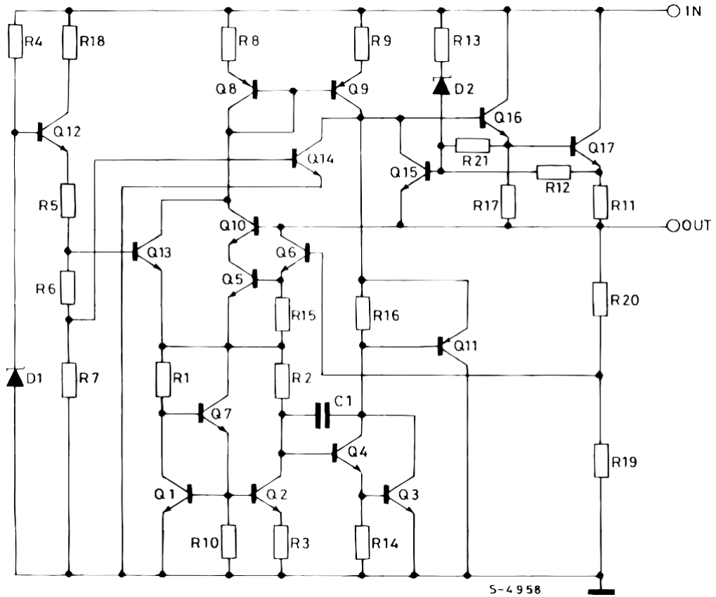
Figure 3. Schematic diagram
