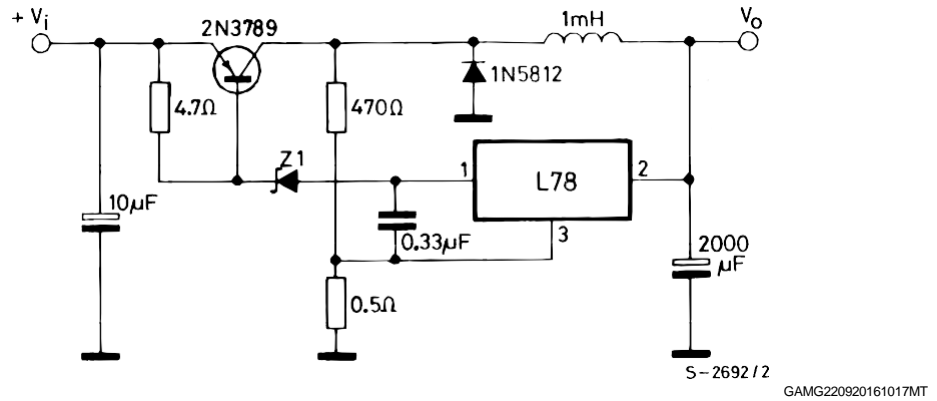
Figure 19. High input voltage circuit (configuration 1)
